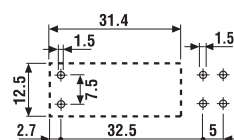
45.91...0310 (1 NO/SPST-NO)
