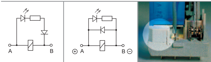
C: 选项3、5、54 LED (AC)
